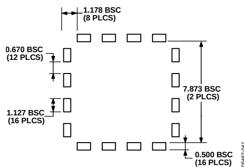
Figure 5. Example Pad Layout
