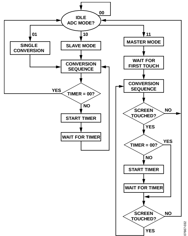
Figure 32. Conversion Modes
