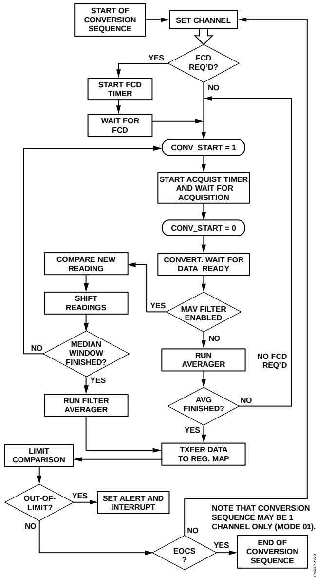
Figure 33. Conversion Sequence
