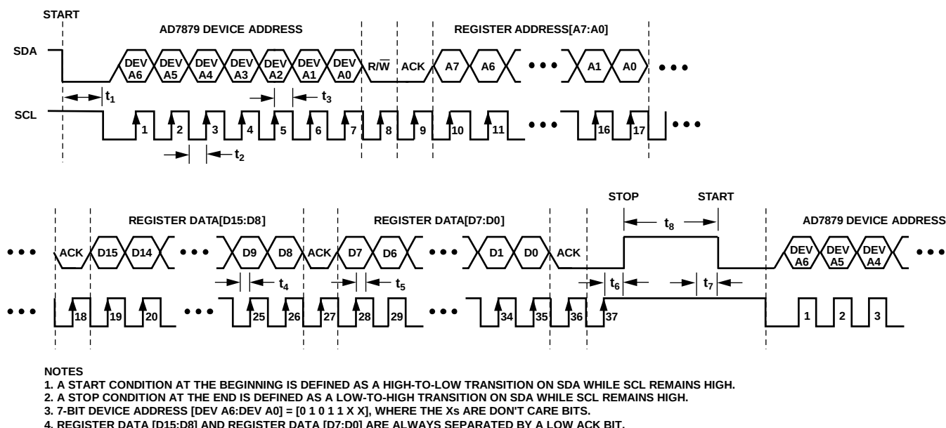
Figure 42. Example of I²C Timing for Single Register Write Operation
