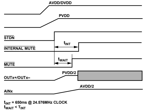
Figure 44. Power-Up Sequence, t_{WAIT} < t_{INT}
