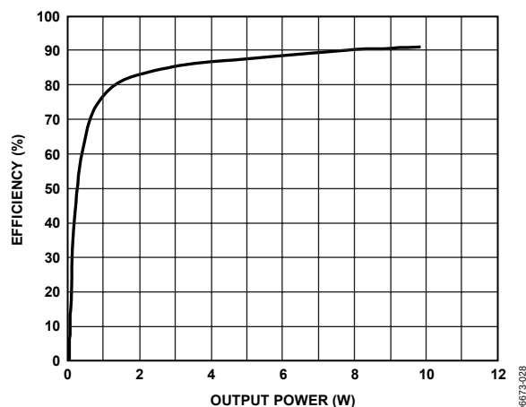
Figure 28. Efficiency vs. Output Power, 12 V, 8 \Omega
