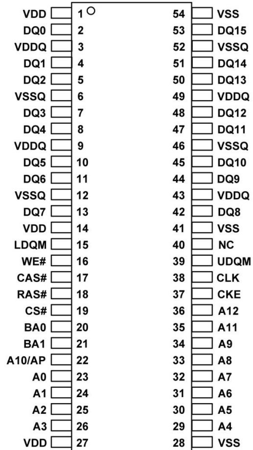
Figure 1. Pin Assignment (Top View)
