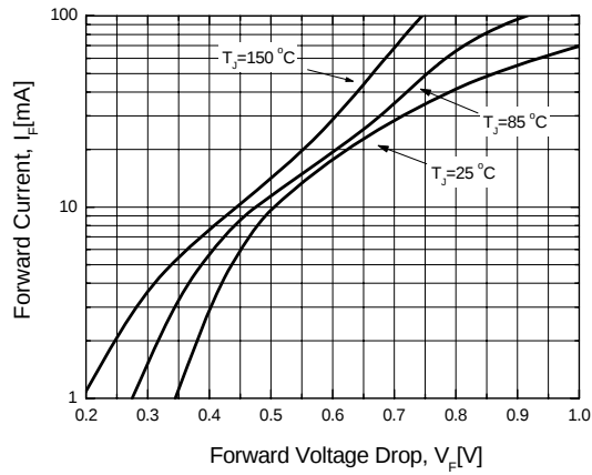
Figure 1. Forward Current Characteristics
