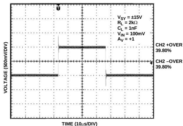
Figure 36. AD8671 Capacitive Load Drive
