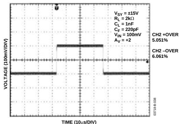
Figure 38. Compensated Load Drive
