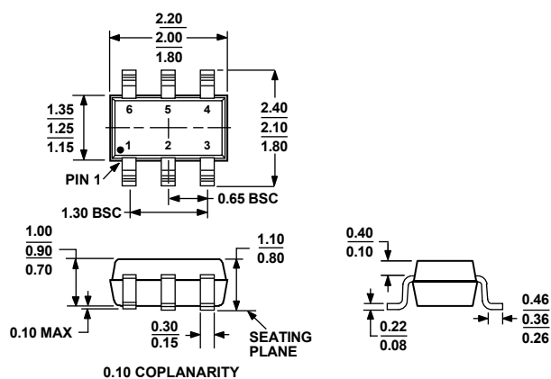
Figure 51. 6-Lead Thin Shrink Small Outline Transistor Package [SC70] (KS-6) Dimensions shown in millimeters
