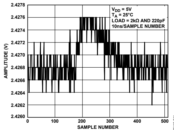
Figure 33. Digital Feedthrough
