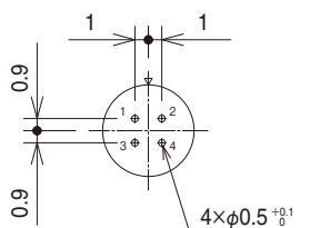
Size 7, 4 conductors
