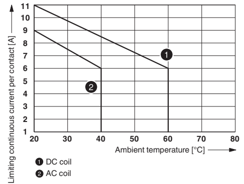
Contact derating
