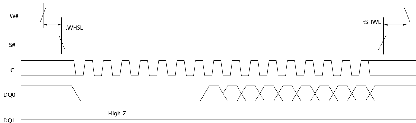
Figure 27: Write Protect Setup and Hold Timing
