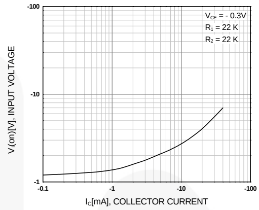
Figure 2. Input-On Voltage
