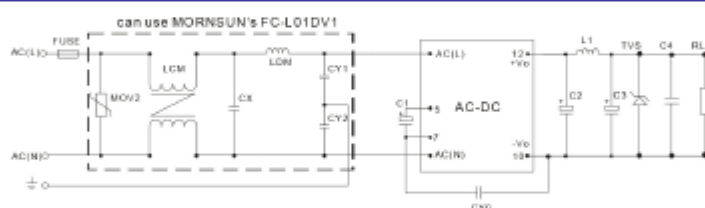
(Figure 3): series recommended circuit for applications which require higher EMC standard
