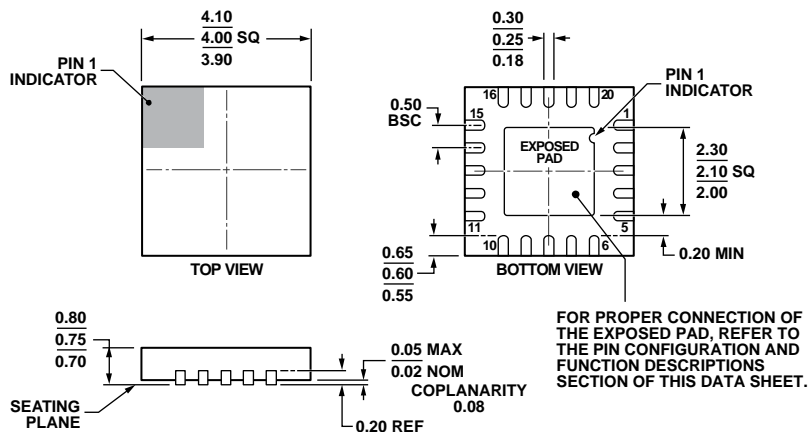
Figure 12. 20-Lead Lead Frame Chip Scale Package [LFCSF_WQ] 4 mm x 4 mm Body, Very Very Thin Quad (CP-20-6)
