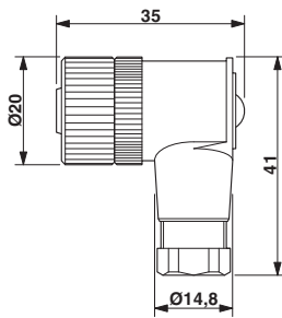
Dimensioned drawing
