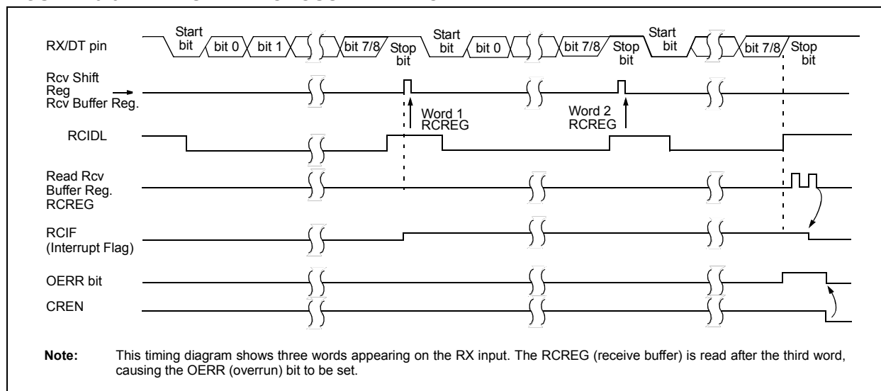
FIGURE 23-5: ASYNCHRONOUS RECEPTION
