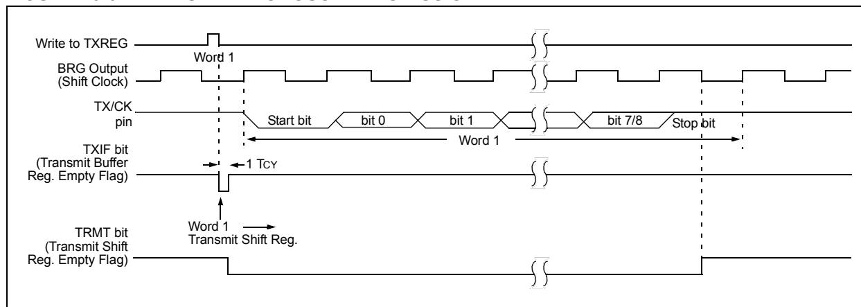
FIGURE 23-3: ASYNCHRONOUS TRANSMISSION
