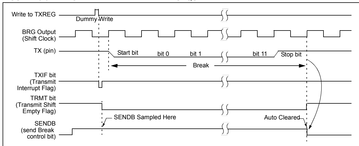
FIGURE 23-9: SEND BREAK CHARACTER SEQUENCE
