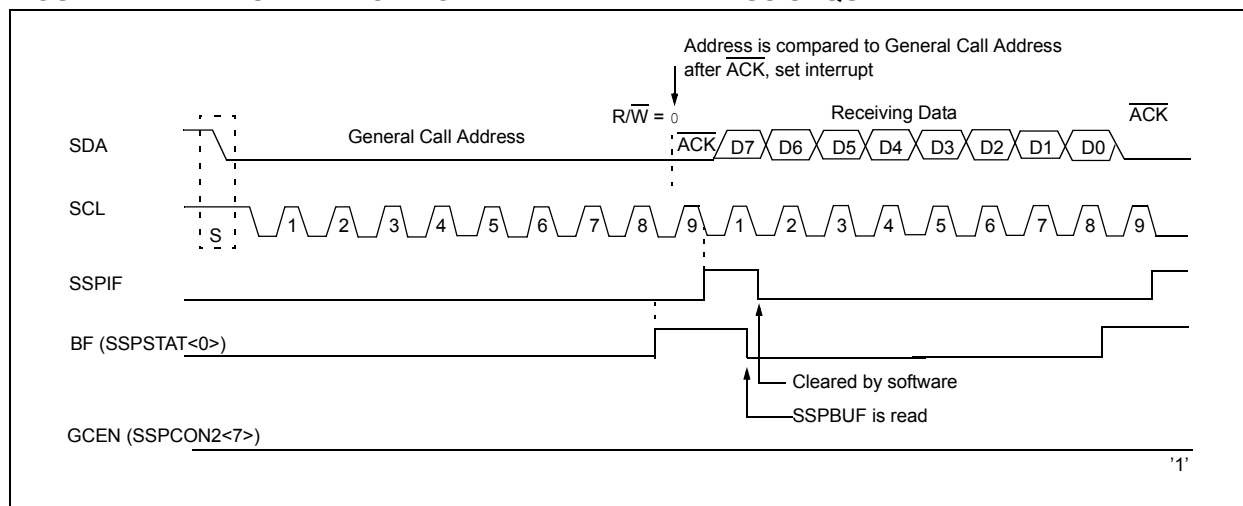
FIGURE 22-24: SLAVE MODE GENERAL CALL ADDRESS SEQUENCE
