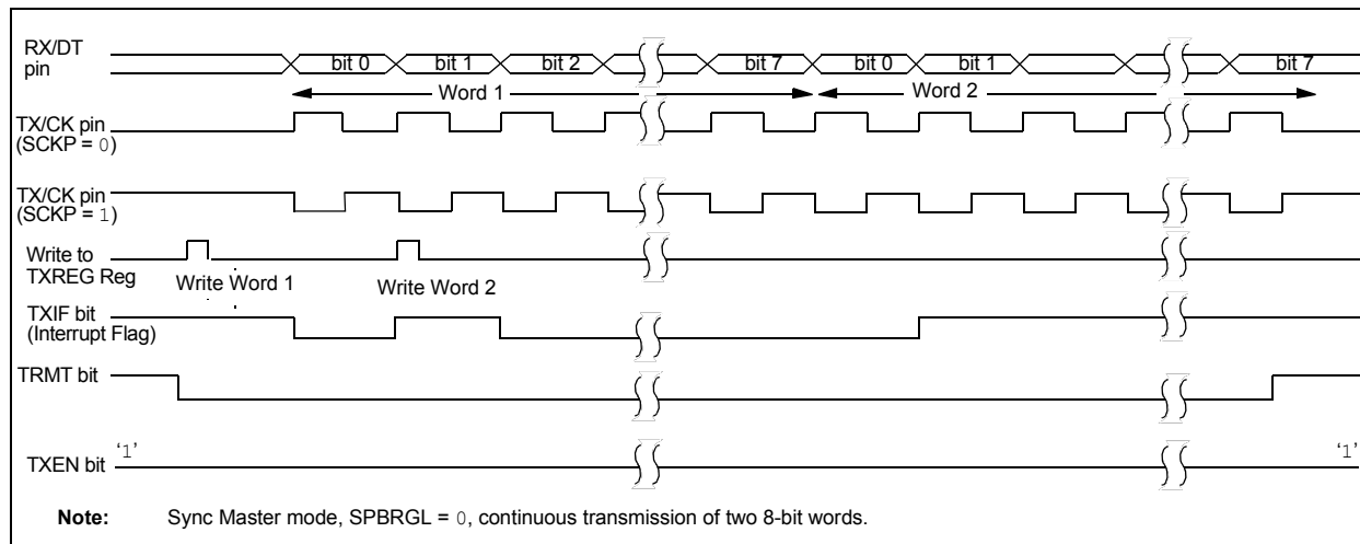
FIGURE 23-10: SYNCHRONOUS TRANSMISSION
