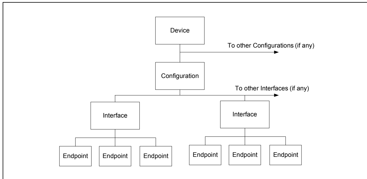
FIGURE 26-11: USB LAYERS
