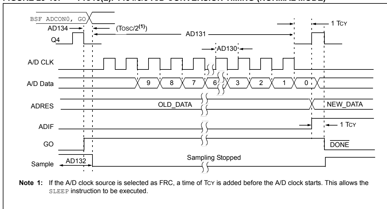
FIGURE 29-10: PIC16(L)F1454/5/9 A/D CONVERSION TIMING (NORMAL MODE)
