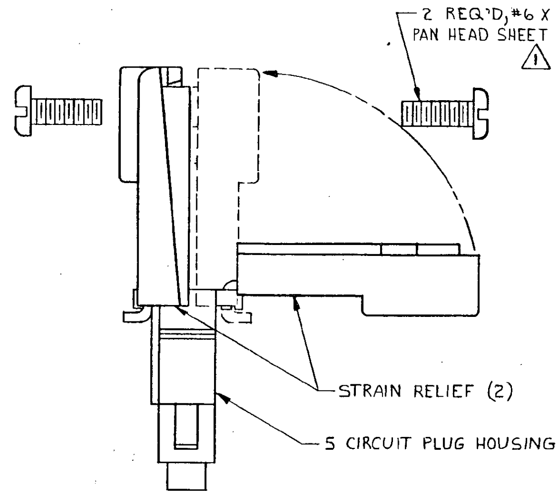
ASSEMBLY DETAILS
