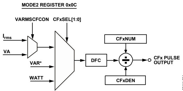
Figure 79. Energy-to-Frequency Conversion
