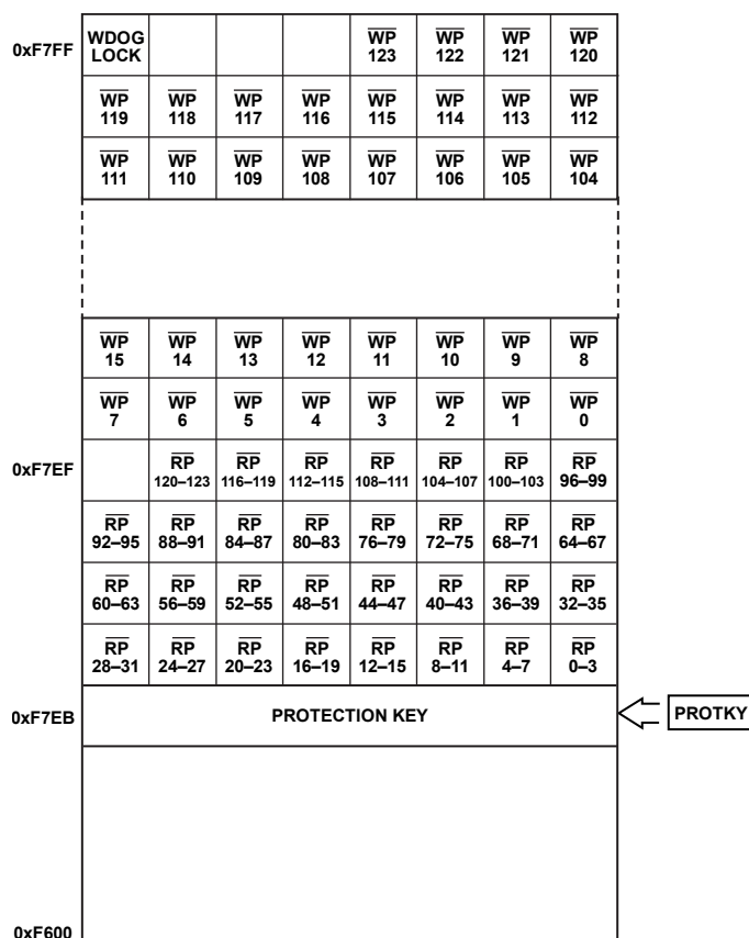
Figure 96. Flash Protection in Page 124
