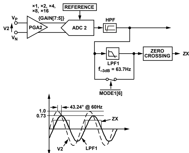
Figure 55. Zero-Crossing Detection on the Voltage Channel
