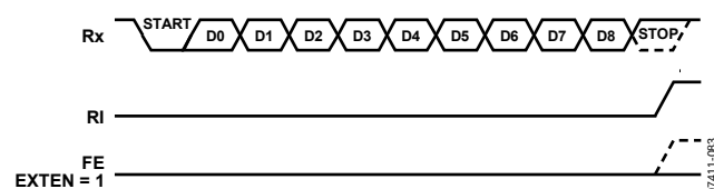
Figure 109. UART Timing in Mode 2 and Mode 3
