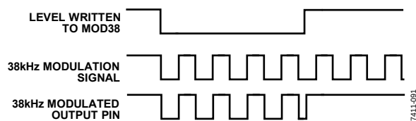
Figure 118. 38 kHz Modulation
