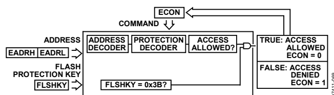
Figure 94. Flash Memory Read/Write/Erase Protection Block Diagram
