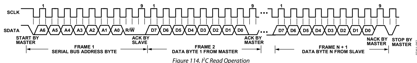
Figure 114. I 2 C Read Operation
