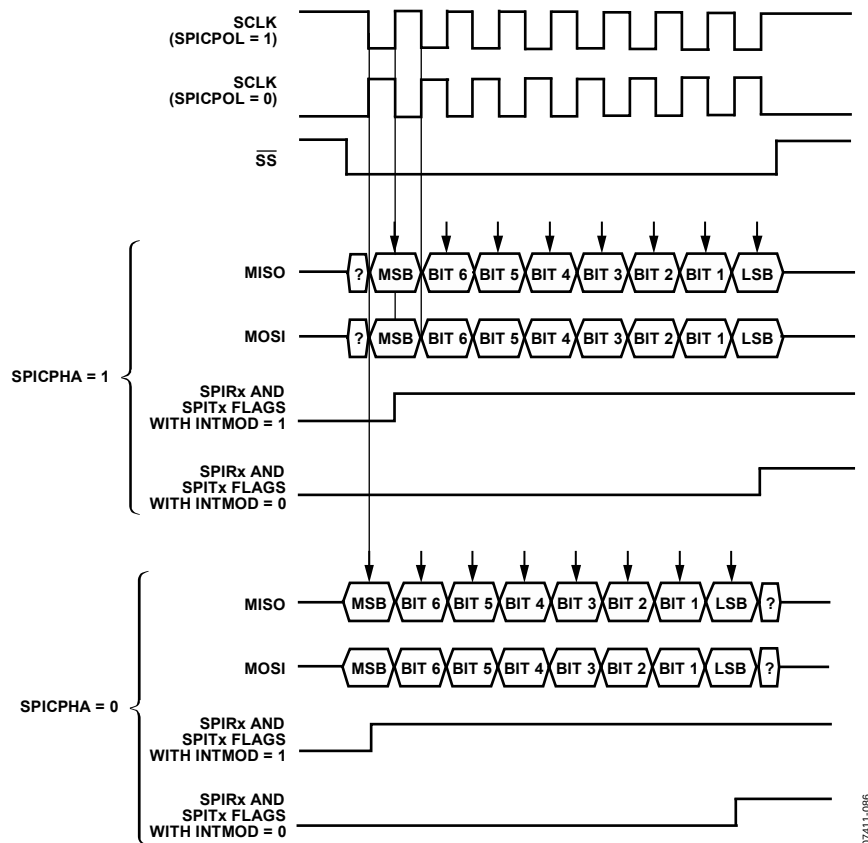
Figure 113. SPI Timing Configurations
