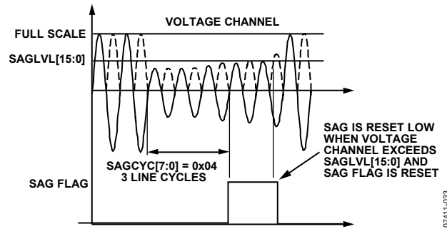
Figure 57. SAG Detection
