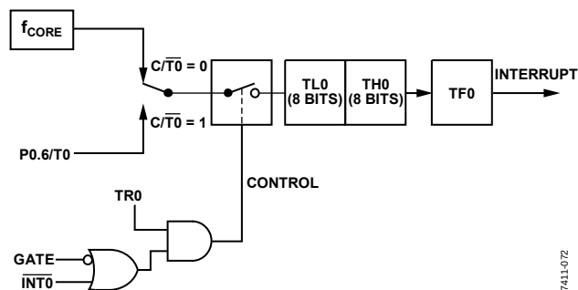
Figure 98. Timer/Counter 0, Mode 1
