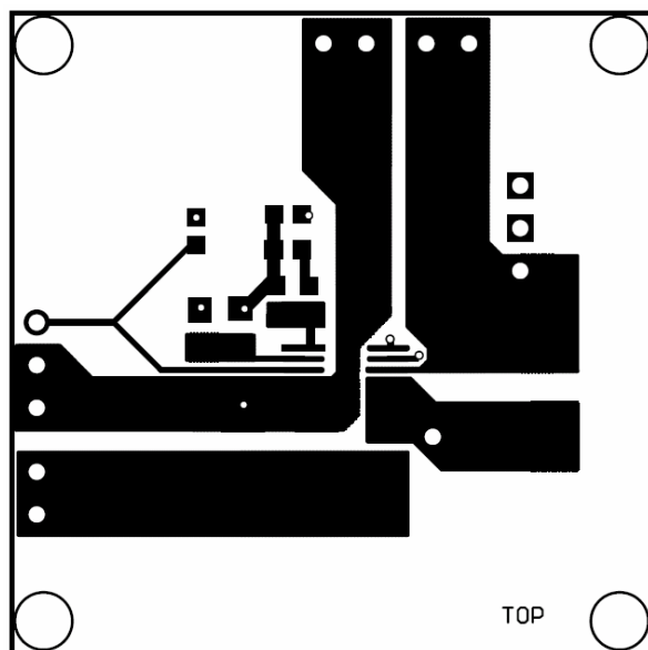
Figure 4. Top Layer
