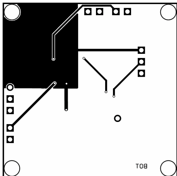
Figure 2. Bottom Layer
