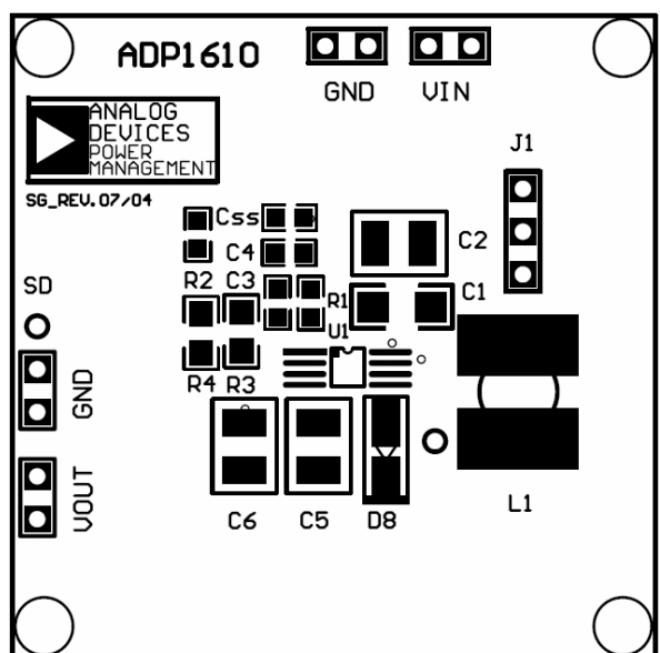
Figure 3. Top Silkscreen
