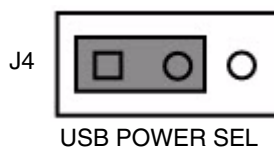
Figure 2-4. Jumper Placement for USB OSBDM Source
