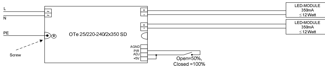
Figure 3: Connection of a switch
