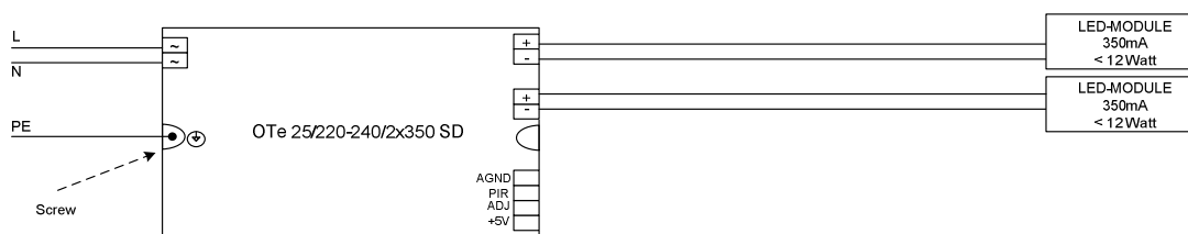
Figure 1: Standard configuration
