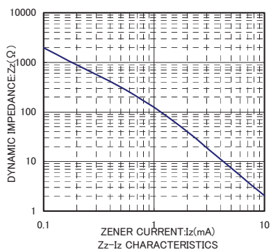
ZENER CURRENT: I_Z (mA) Z Z -I Z CHARACTERISTICS
