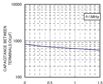
REVERSE VOLTAGE: V_R (V) V R -C t CHARACTERISTICS
