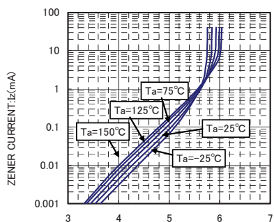
ZENER VOLTAGE: V_Z (V) Z Z -I Z CHARACTERISTICS
