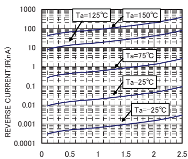
REVERSE VOLTAGE: V_R (V) V R -I R CHARACTERISTICS
