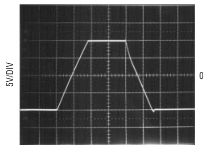
Large-Signal Transient Response V_S = \pm 15V
