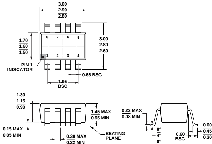
Figure 53. 8-Lead Small Outline Transistor Package [SOT-23] (RJ-8)
