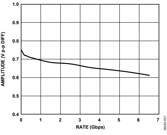
Figure 27. Output Amplitude vs. Rate
