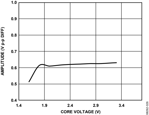
Figure 26. Output Amplitude (Default Setting) vs. V_{CC}
