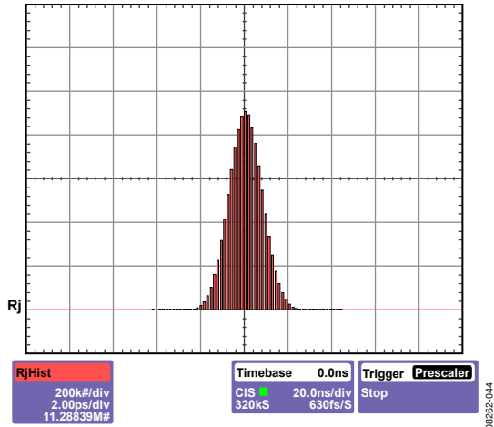
Figure 24. Random Jitter Histogram
