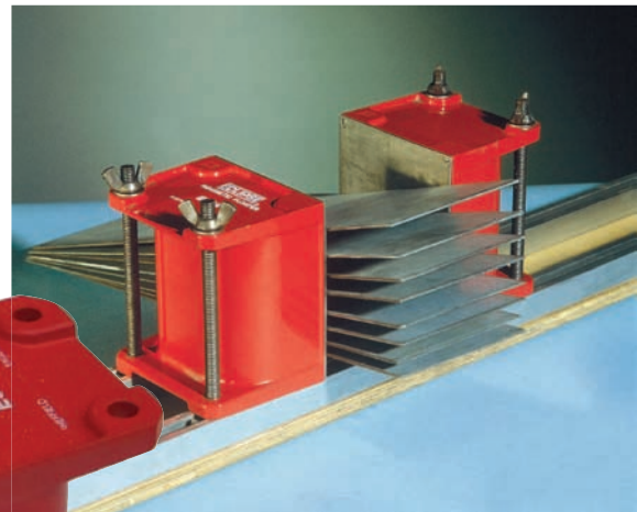
Standard magnetic sheet separator
