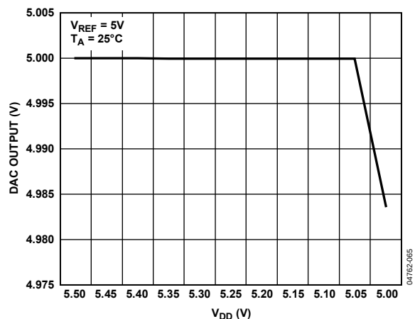
Figure 29. Typical Output Voltage vs. Supply Voltage
