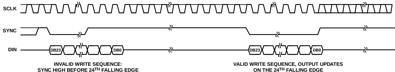
Figure 41. SYNC Interrupt Facility
