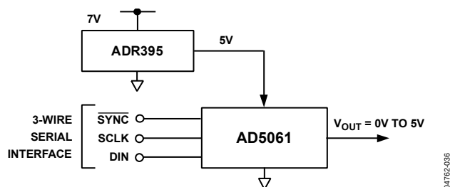
Figure 46. ADR395 as Reference to the AD5061
