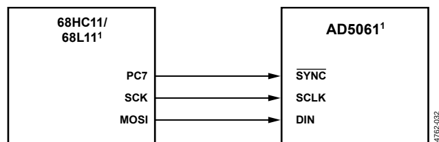
Figure 42. AD5061-to-68HC11/68L11 Interface
