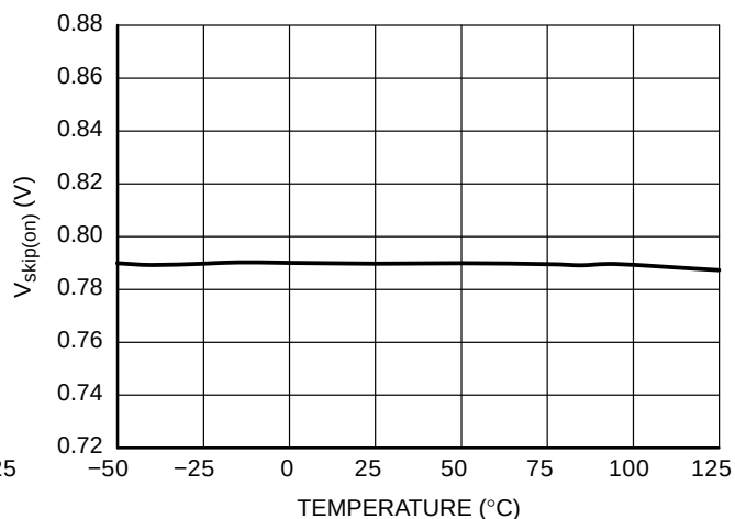
Figure 30. FB Pin Skip-Out Level V_{skip(out)}
