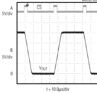
BIPOLAR SETTLING TIME ( C_{LOAD} = 250pF , R_{LOAD} = 2k\Omega )
