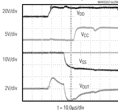
BIPOLAR STARTUP RESPONSE, C_{LOAD} = 10\text{pF}
