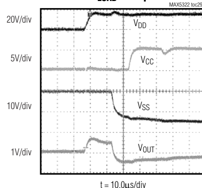
BIPOLAR STARTUP RESPONSE, C_{LOAD} = 230\text{pF}
