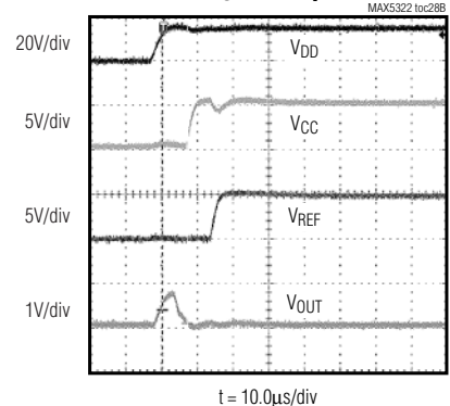
UNIPOLAR STARTUP RESPONSE, C_{LOAD} = 230\text{pF}
