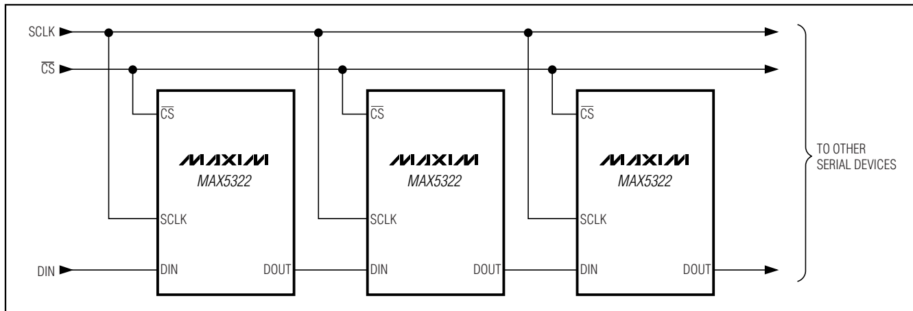
Figure 7. Daisy-Chaining Devices
