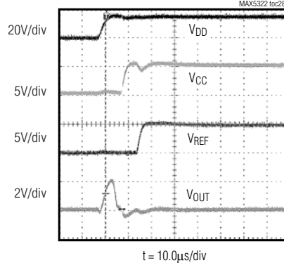
UNIPOLAR STARTUP RESPONSE, C_{LOAD} = 10\text{pF}
