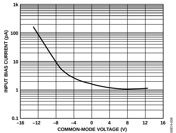
Figure 8. Input Bias Current vs. Common-Mode Voltage; V_S = \pm 15V
