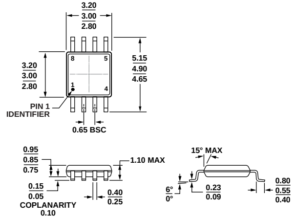
Figure 53. 8-Lead Mini Small Outline Package [MSOP] (RM-8)
