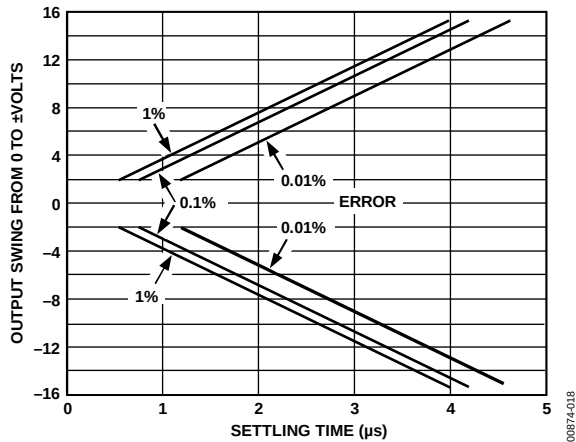
Figure 18. Output Swing and Error vs. Settling Time
