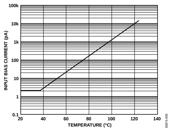
Figure 9. Input Bias Current vs. Temperature; V_S = 5V, V_{CM} = 0V
