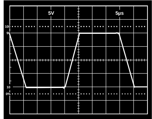
Figure 32. Large Signal Response Unity-Gain Follower; V_S = \pm 15 V, R_L = 10 kΩ
