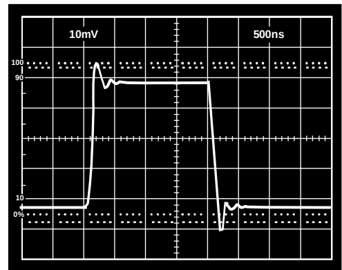
Figure 33. Small Signal Response Unity-Gain Follower; V_S = \pm 15 V, R_L = 10 kΩ
