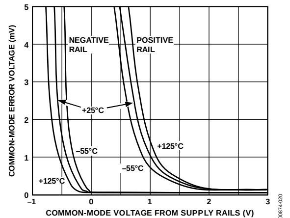
Figure 20. Absolute Common-Mode Error vs. Common-Mode Voltage from Supply Rails ( V_S - V_{CM} )
