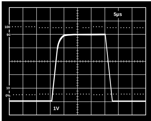
Figure 48. Pulse Response of In-Amp to a 500 mV p-p Input Signal; V_S = 5\text{ V}, 0\text{ V}; \text{Gain} = 0
