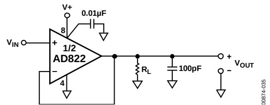
Figure 35. Unity-Gain Follower
