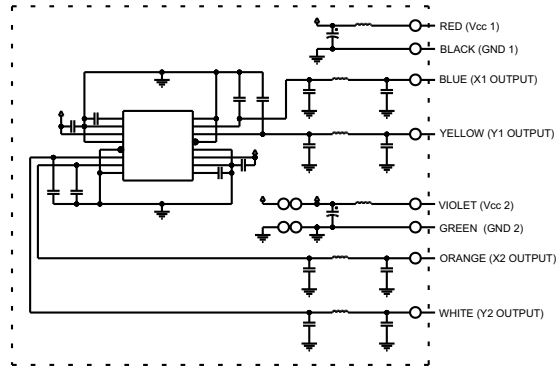
GENERAL SCHEMATIC
