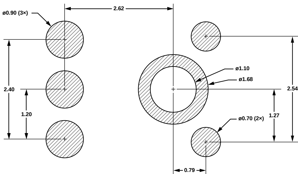
Figure 11. PCB Land Pattern Layout
