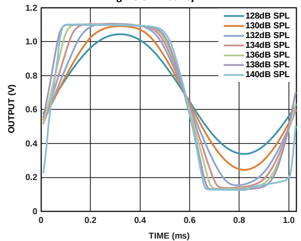
Figure 8. Clipping Characteristics
