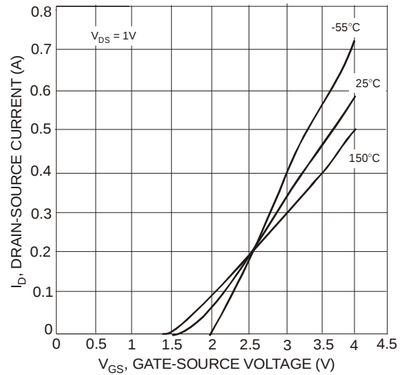
Fig. 2 Transfer Characteristics
