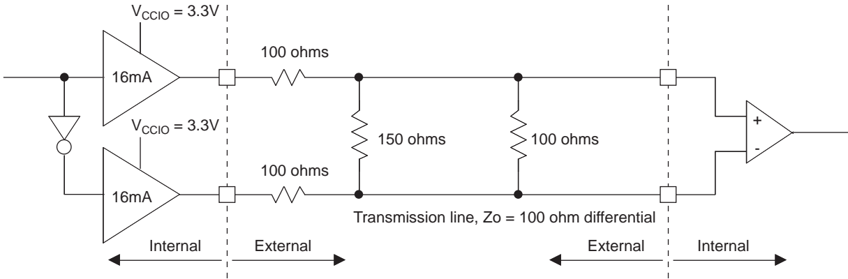
Figure 5. Differential LVPECL
