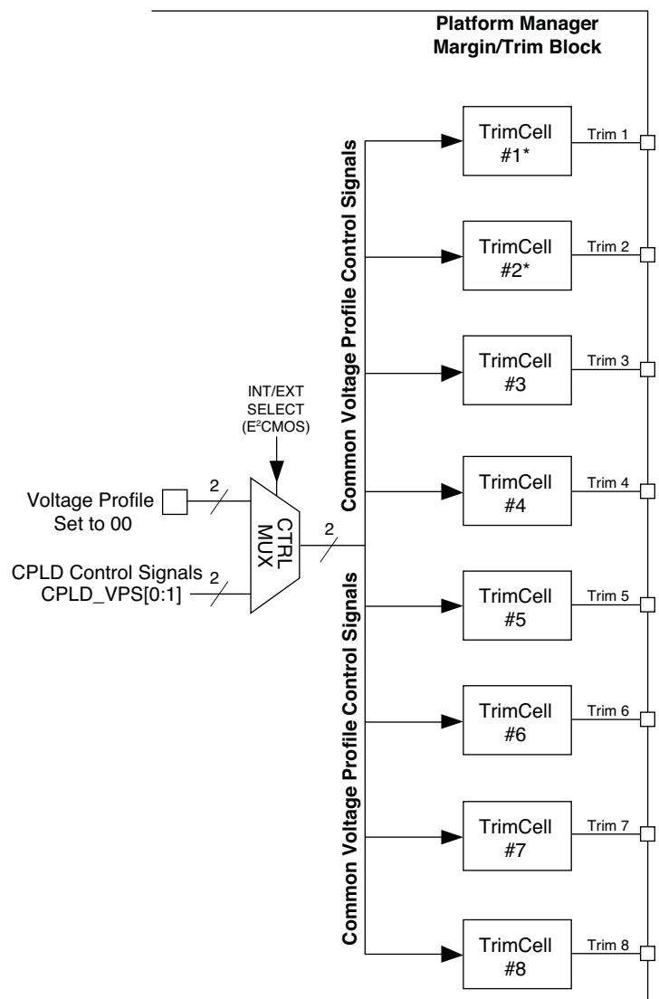
Figure 18. Voltage Profile Control
