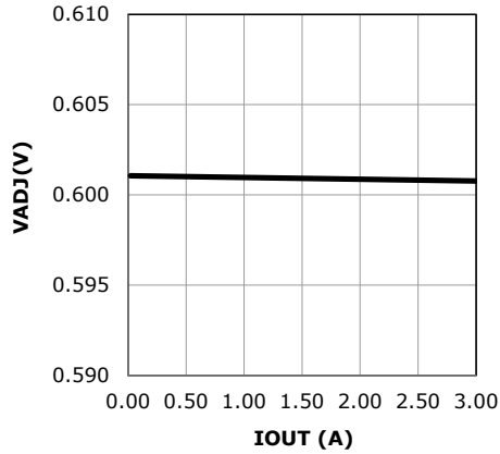
Fig. 4: VADJ versus IOU, 1.5VIN, 1VOUT
