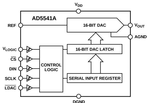
Figure 1. AD5541A
