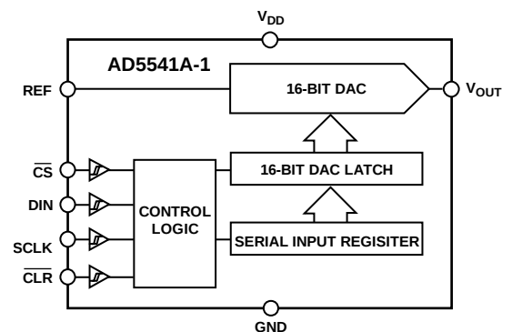
Figure 2. AD5541A-1
