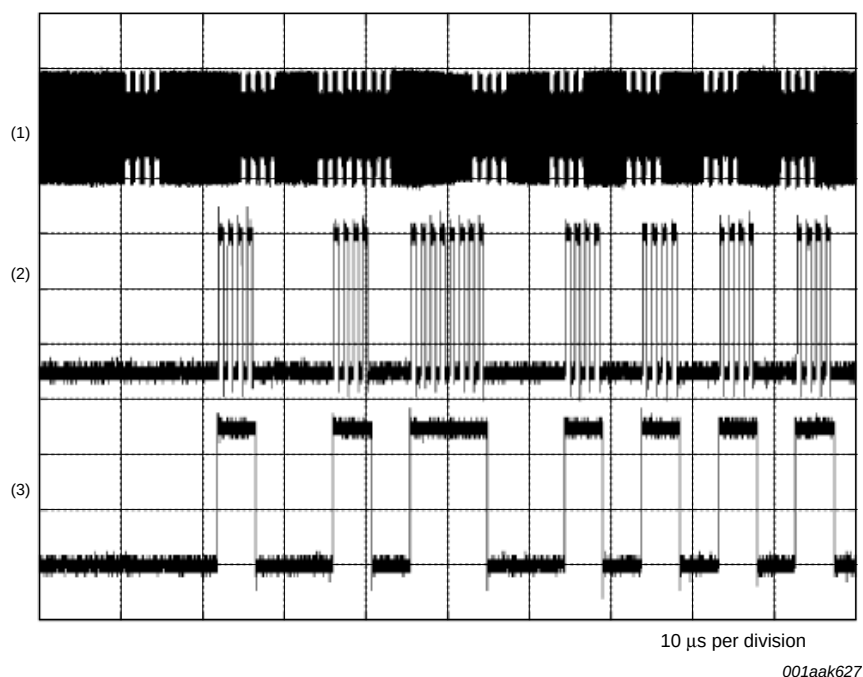
(1) RFOut; 1 V per division. (2) MFOUTSelect[2:0] = 4; Manchester with subcarrier; 2 V per division. (3) MFOUTSelect[2:0] = 5; Manchester; 2 V per division.
