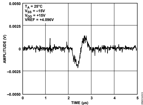
Figure 12. Digital Crosstalk
