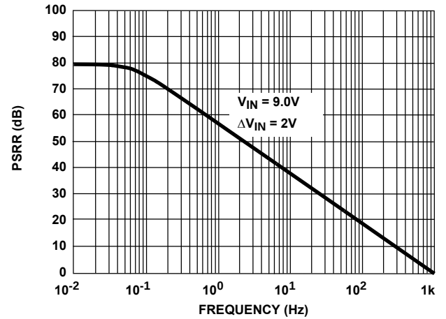
FIGURE 4. NPUT POWER SUPPLY REJECTION RATIO
