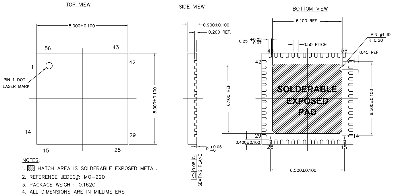
Figure 6. 56-pin QFN ( 8 \times 8 \times 1.0 mm) LT56 6.1 \times 6.1 E-Pad (Sawn) Package Outline, 51-85187
