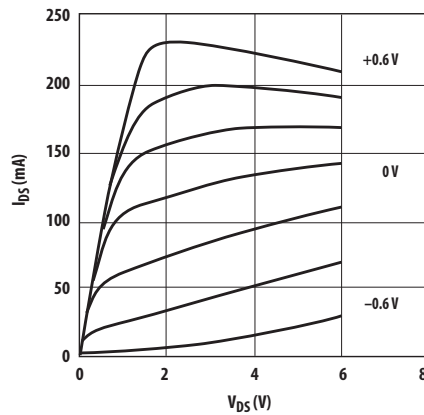
Figure 1. Typical/Pulsed I-V Curves [6] . ( V_{GS} = -0.2\text{V} per step)
