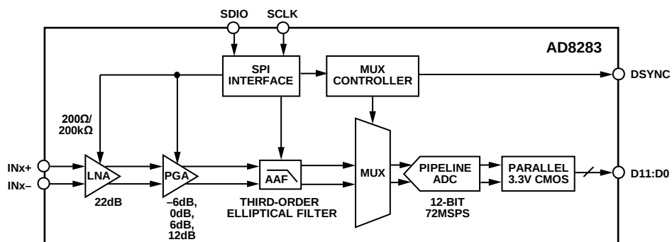
Figure 25. Simplified Block Diagram of a Single Channel
