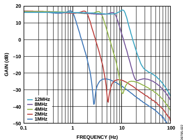
Figure 14. Filter Response
