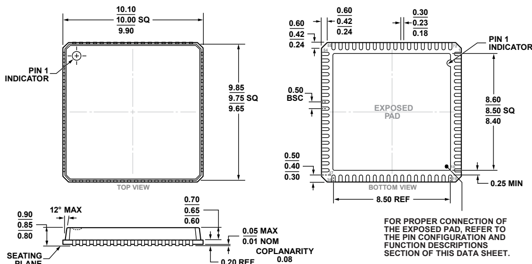
Figure 35. 72-Lead Lead Frame Chip Scale Package [LFCSP_VQ] 10 mm x 10 mm Body, Very Thin Quad (CP-72-5) Dimensions shown in millimeters
