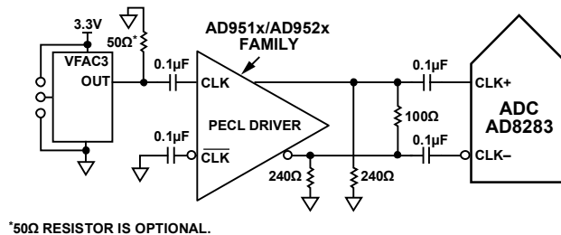
Figure 28. Differential PECL Sample Clock
