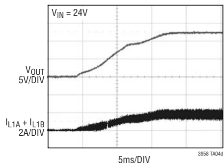
Start-Up Waveforms
