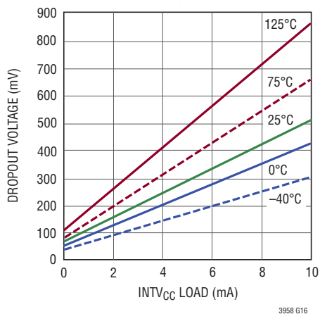
INTV CC Dropout Voltage vs Current, Temperature
