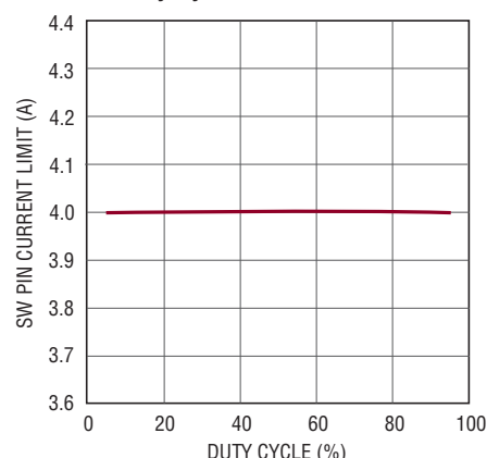
SW Pin Current Limit vs Duty Cycle
