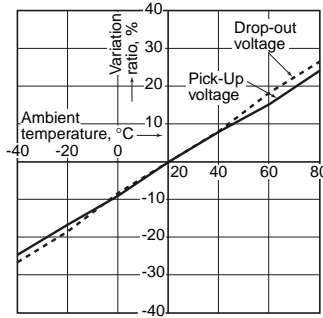
1.-(2) Ambient temperature characteristics (20 A type)
