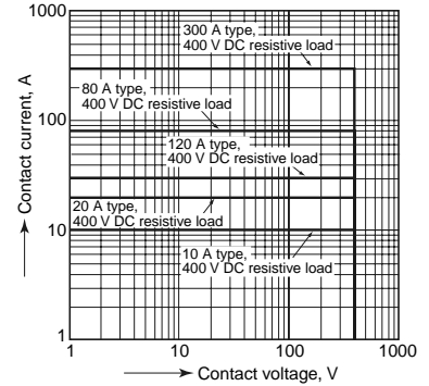
5. Carrying performance curve (80°C 176°F)
