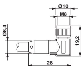
Socket M8 x 1, angled
