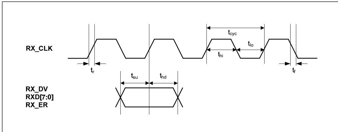
Figure 14. GMII Receive Timing - Data Input to MAC
