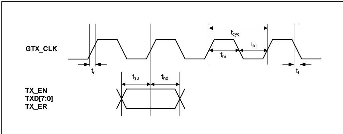
Figure 13. GMII Transmit Timing - Data Input to PHY
