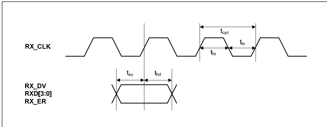
Figure 16. MII Receive Timing - Data Input to MAC
