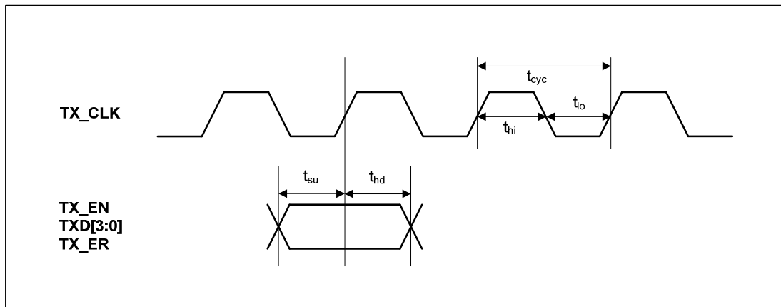
Figure 15. MII Transmit Timing - Data Input to PHY
