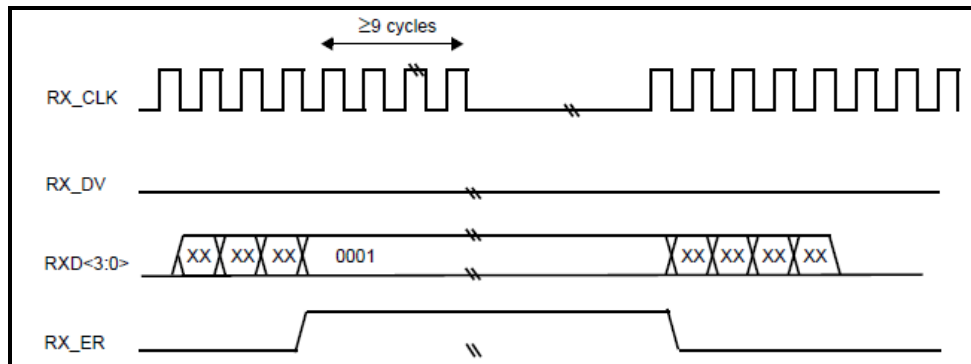
Figure 12. LPI Transition – MII (100Mbps) Receive
