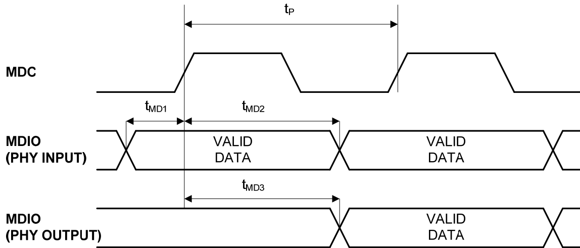
Figure 18. MDC/MDIO Timing
