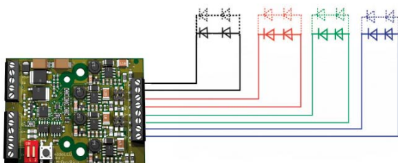
Example of an LED group wiring schematic
