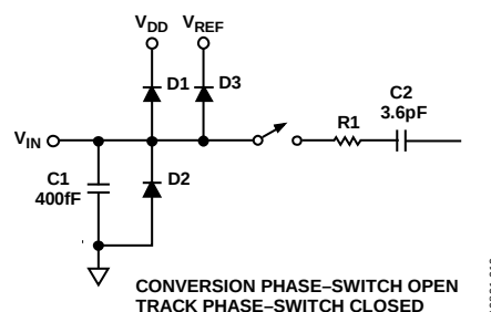
Figure 43. Equivalent Analog Input Circuit
