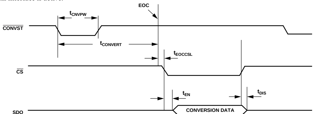
Figure 52. Serial Interface Read Timing in Normal Mode
