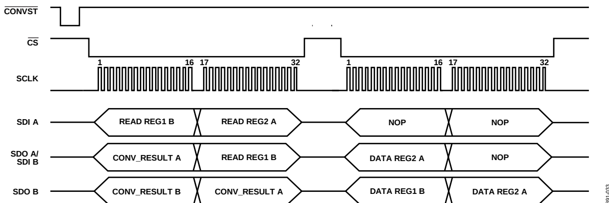
Figure 58. Single Register Read in a Two-Slave Daisy-Chain Mode Configuration
