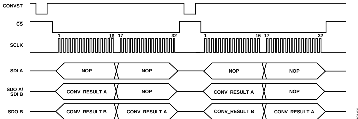
Figure 56. Conversion in a Two-Slave Daisy-Chain Mode Configuration
