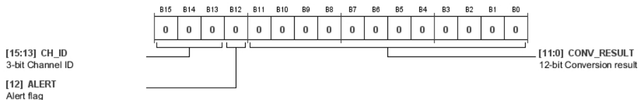
Figure 46. Conversion Result Register
