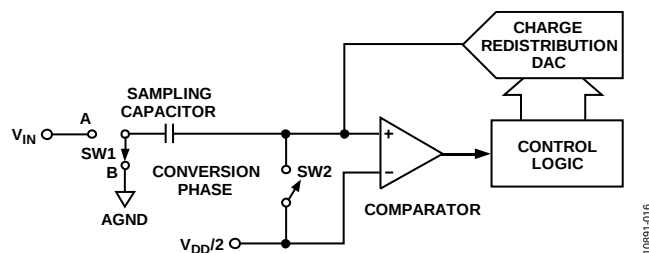
Figure 41. ADC Conversion Phase
