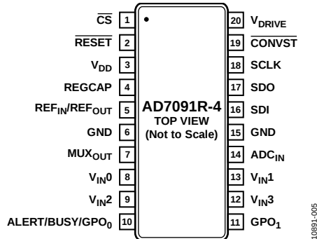
Figure 7. 4-Channel, 20-Lead TSSOP Pin Configuration
