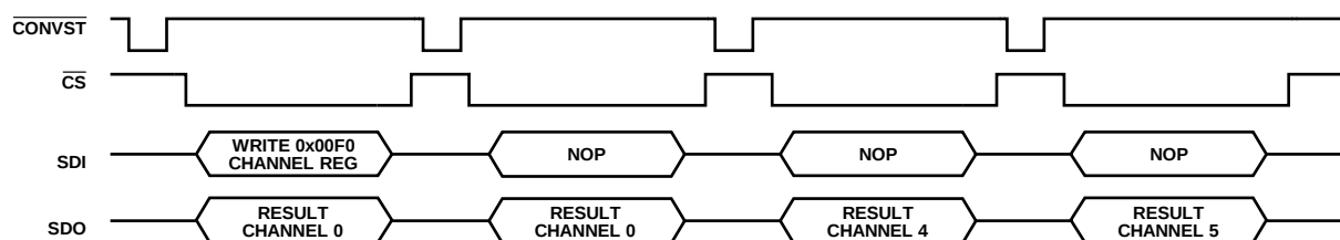
Figure 53. Channel Sequencer
