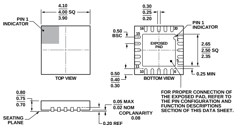
Figure 63. 20-Lead Lead Frame Chip Scale Package [LFCSP_WQ] 4 mm × 4 mm Body, Very Very Thin Quad (CP-20-10) Dimensions shown in millimeters
