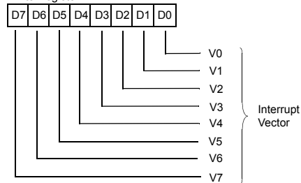
Write Register 2
