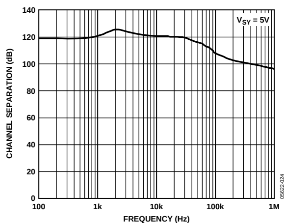
Figure 27. Channel Separation
