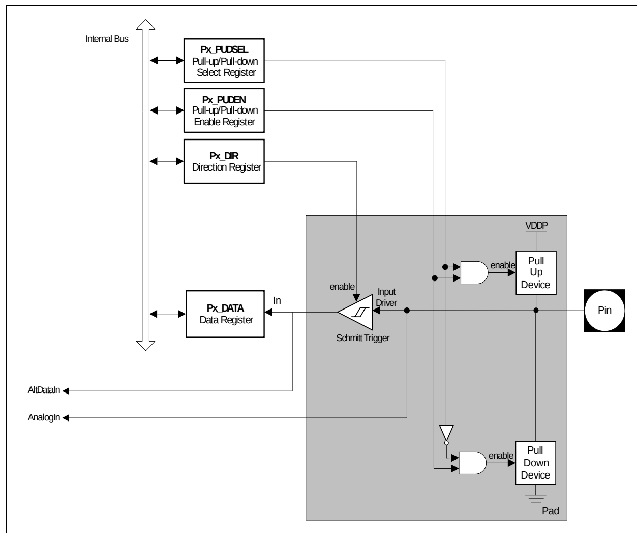
Figure 20 General Structure of Input Port
